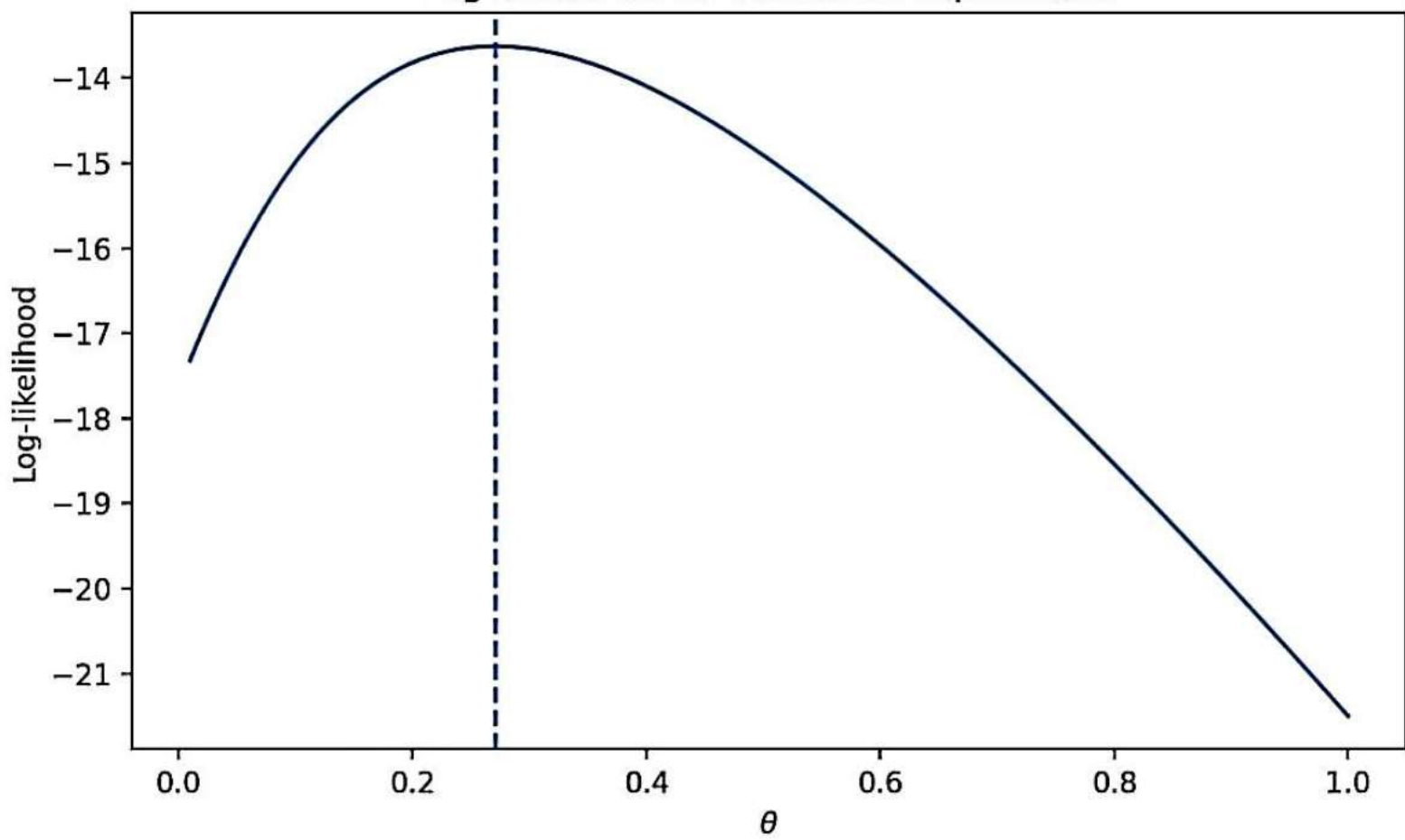
Log-likelihood for truncated exponential
